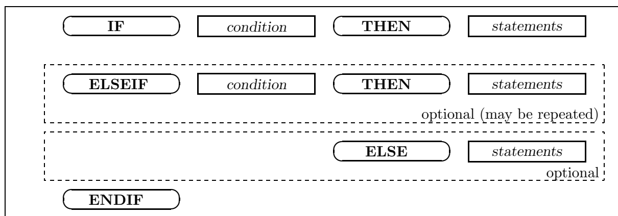
Figure 11: The IF statement.
