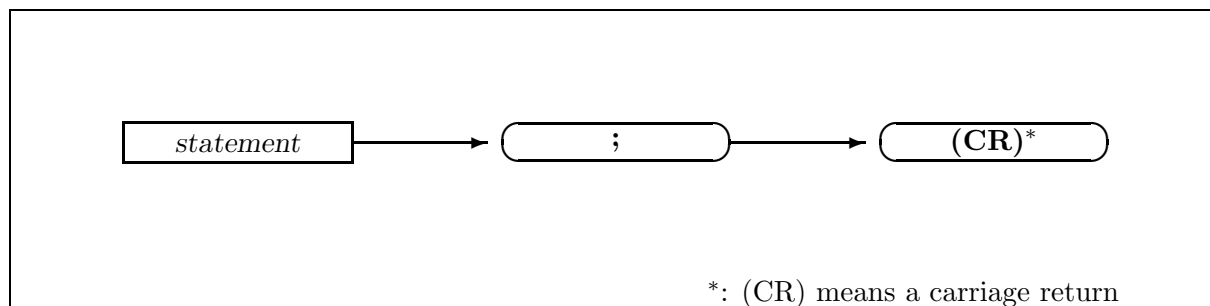
Figure 2: Definition of an instruction.
