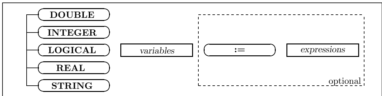
Figure 3: The declaration statement.
