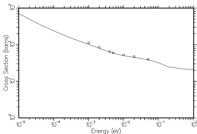
Figure 98: The computed cross section for liquid methane at 100K (solid) is compared to experimental data at 110K (squares) by Whittemore and by Rogalska as quoted by Agrawal and Yip.
