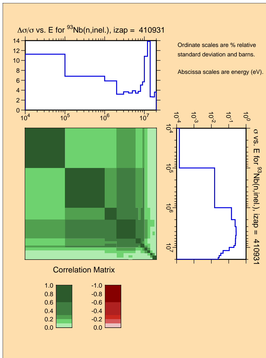
Figure 44: Example of radioactive nuclide production covariances.
