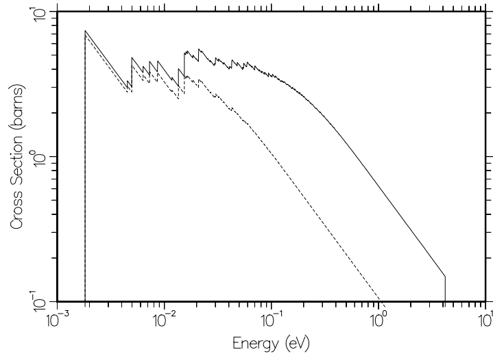
Figure 76: The coherent elastic cross section for graphite at temperatures of 293.6K (solid) and 2000K (dashed) showing the Bragg peaks. Note that the 293.6K cross section near the 4 eV breakpoint is still an appreciable part of the 4.74 barn free cross section.
