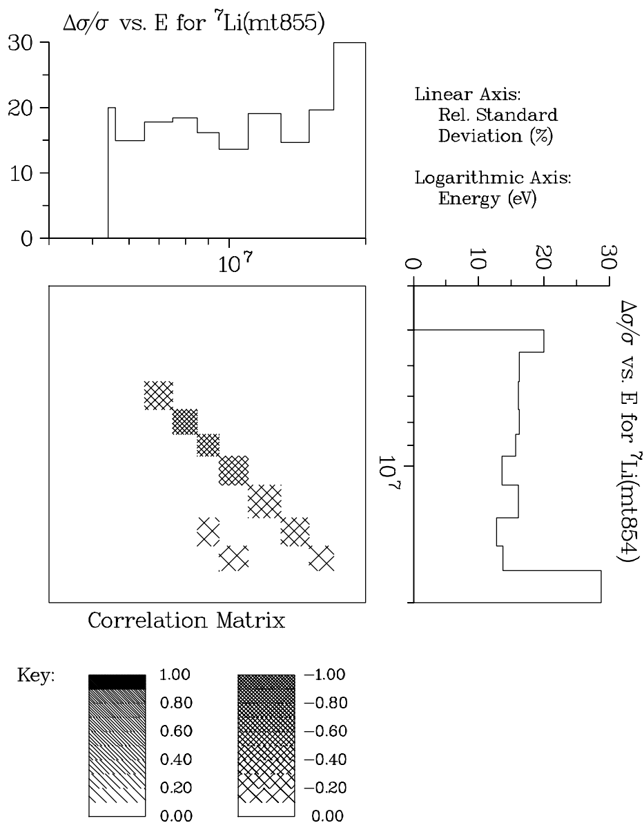
Figure 47: Covariance data for {}^7\text{Li} (MT854) with {}^7\text{Li} (MT855).
