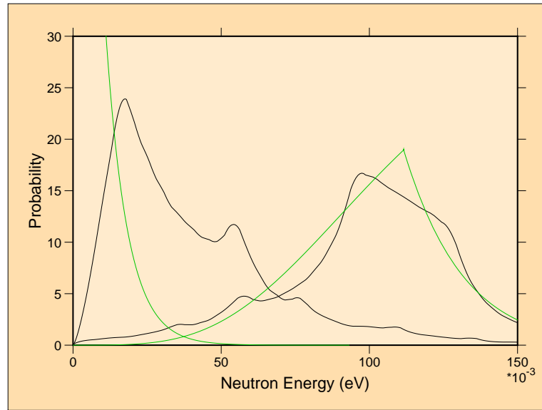
Figure 17: Adaptive reconstruction of two of the emission curves for graphite at 293.6K ( E=.00016 eV to the left, and E=.1116 eV to the right). Note the presence of excitation features from the phonon frequency spectrum for both upscatter and downscatter. The breaks in the curves are due to \beta interpolation in S(\alpha, \beta) and not to the tolerances in the reconstruction process. The green curves are the corresponding free gas results.
