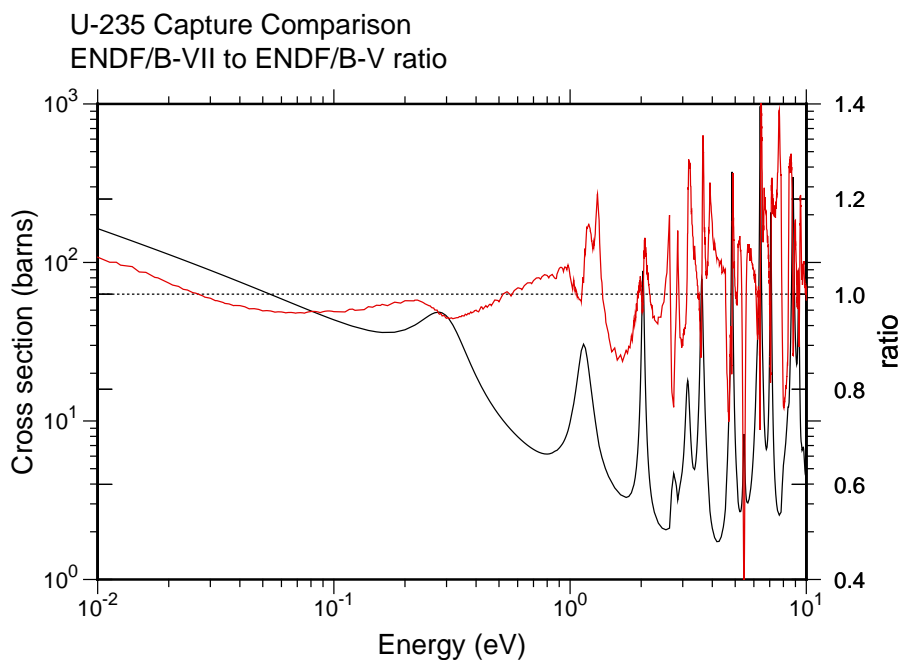
Figure 65: Using a right-hand axis to plot the ratio of the ENDF/B-VII.0 capture cross section for ^{235}\text{U} to the ENDF/B-V value. The black curve is the ENDF/B-V cross section, and the red curve is the ratio (right-hand axis).
