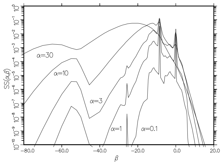
Figure 102: Script-S for para-hydrogen at 20K is shown as a function of \beta for several \alpha values.
