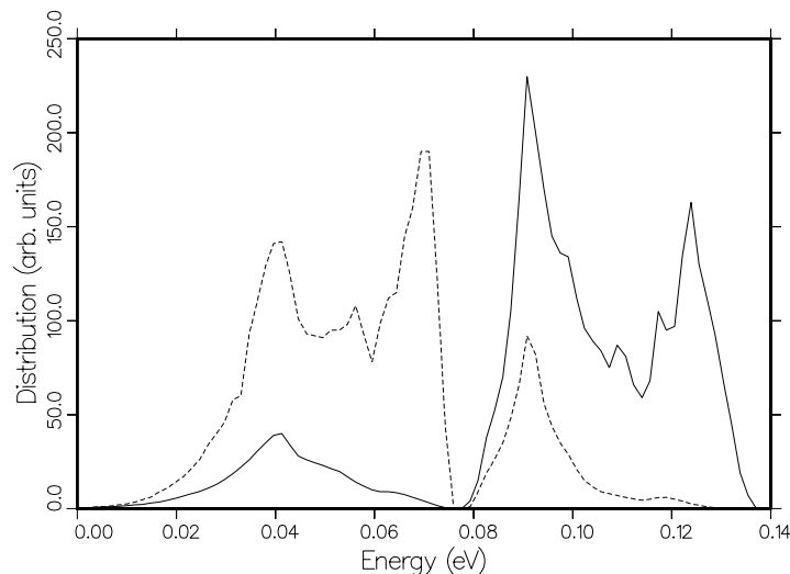
Figure 78: The frequency spectr \rho(\epsilon) used for Be in BeO (solid) and O in BeO (dashed).
