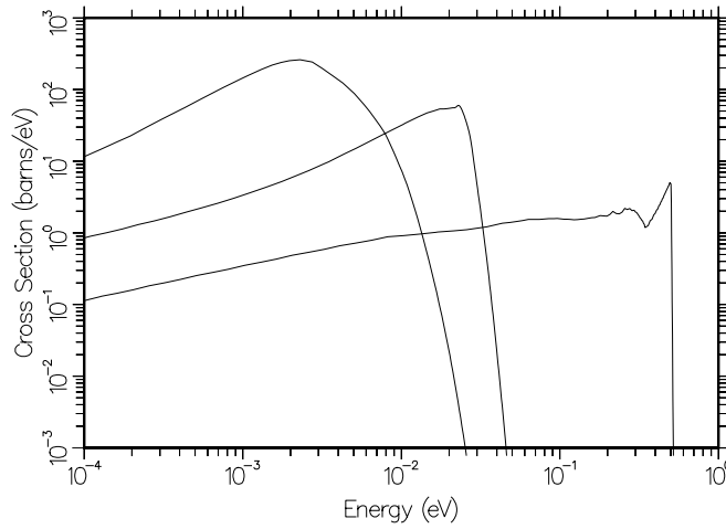
Figure 94: Neutron spectra \sigma(E \rightarrow E') for solid methane shown as functions of outgoing neutron energy E' for E = 0.0001 eV, 0.0253 eV, and 0.503 eV.
