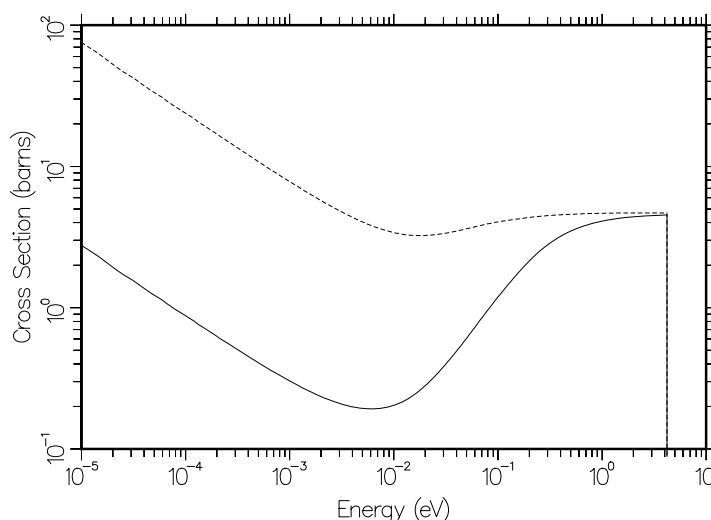
Figure 77: The incoherent inelastic cross section for graphite at temperatures of 293.6K (solid) and 2000K (dashed). A comparison of the two curves near the 4 eV breakpoint shows that the 293.6K cross section still has not reached the 4.74 barn free cross section. However, the sum of the elastic and inelastic components does equal the free value.
