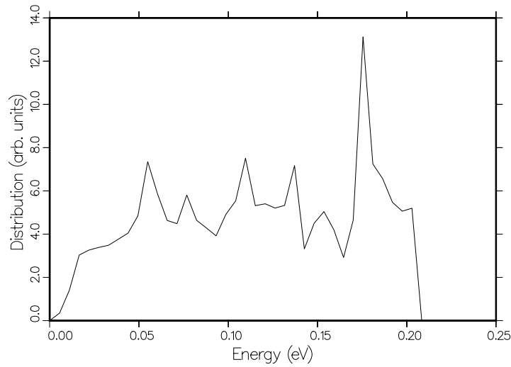
Figure 75: The phonon frequency spectrum \rho(\epsilon) used for graphite.
