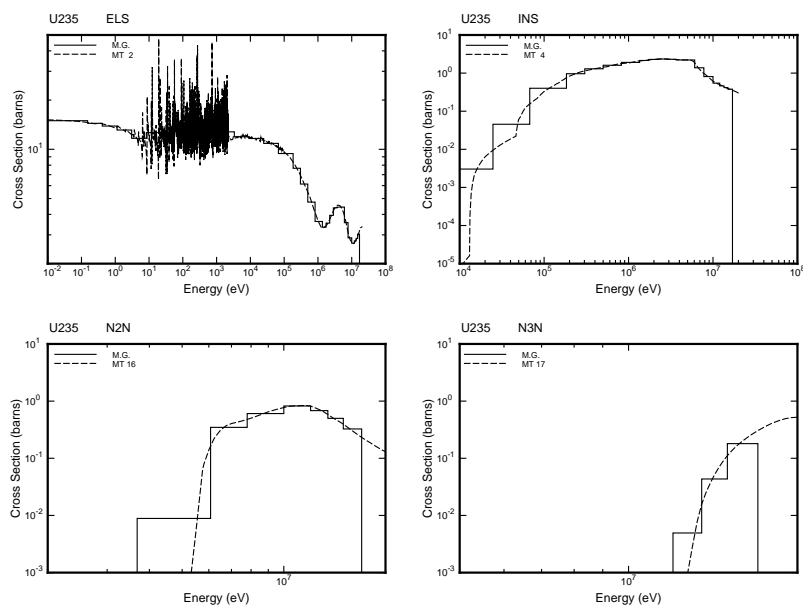
Figure 54: An example of DTFR plotting using ifilm=2 for ENDF/B-VI ^{235}\text{U} for some of the standard edits with iedit=1 .
