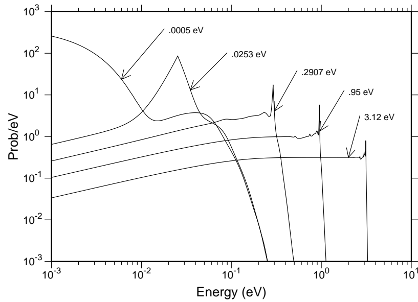
Figure 82: Incoherent inelastic spectra for several incident energies for H in H 2 O.
