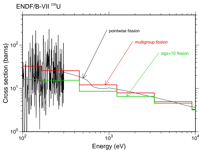
Figure 64: Multigroup fission cross sections of ENDF/B-VII.0 ^{235}\text{U} for infinite dilution and a 10-barn background compared with the corresponding pointwise cross section.
