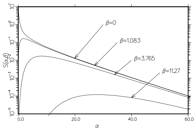
Figure 97: S(\alpha, \beta) curves for liquid methane. Note the diffusive behavior at low \alpha and \beta .
