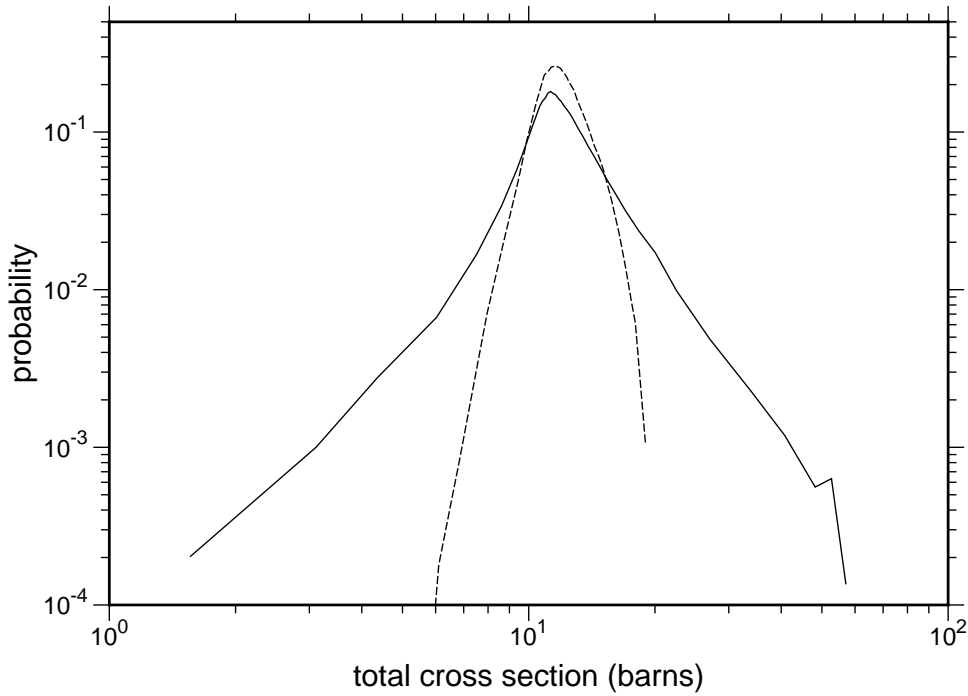
Figure 72: The probability distribution for the total cross section at 20 keV (solid) and 140 keV (dashed) in the unresolved resonance range of ^{238}\text{U} .
