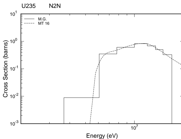
Figure 50: An example of DTFR plotting for the (n,2n) reaction of ENDF/B-VI ^{235}\text{U} . This plot was prepared using ifilm=1 and in-table edits. All the threshold reactions are shown using the same energy range to make comparisons easy.
