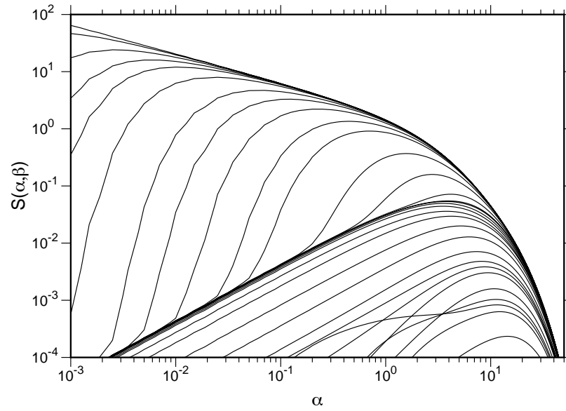
Figure 81: \mathcal{S}(\alpha, -\beta) vs \alpha for a number of \beta values.
