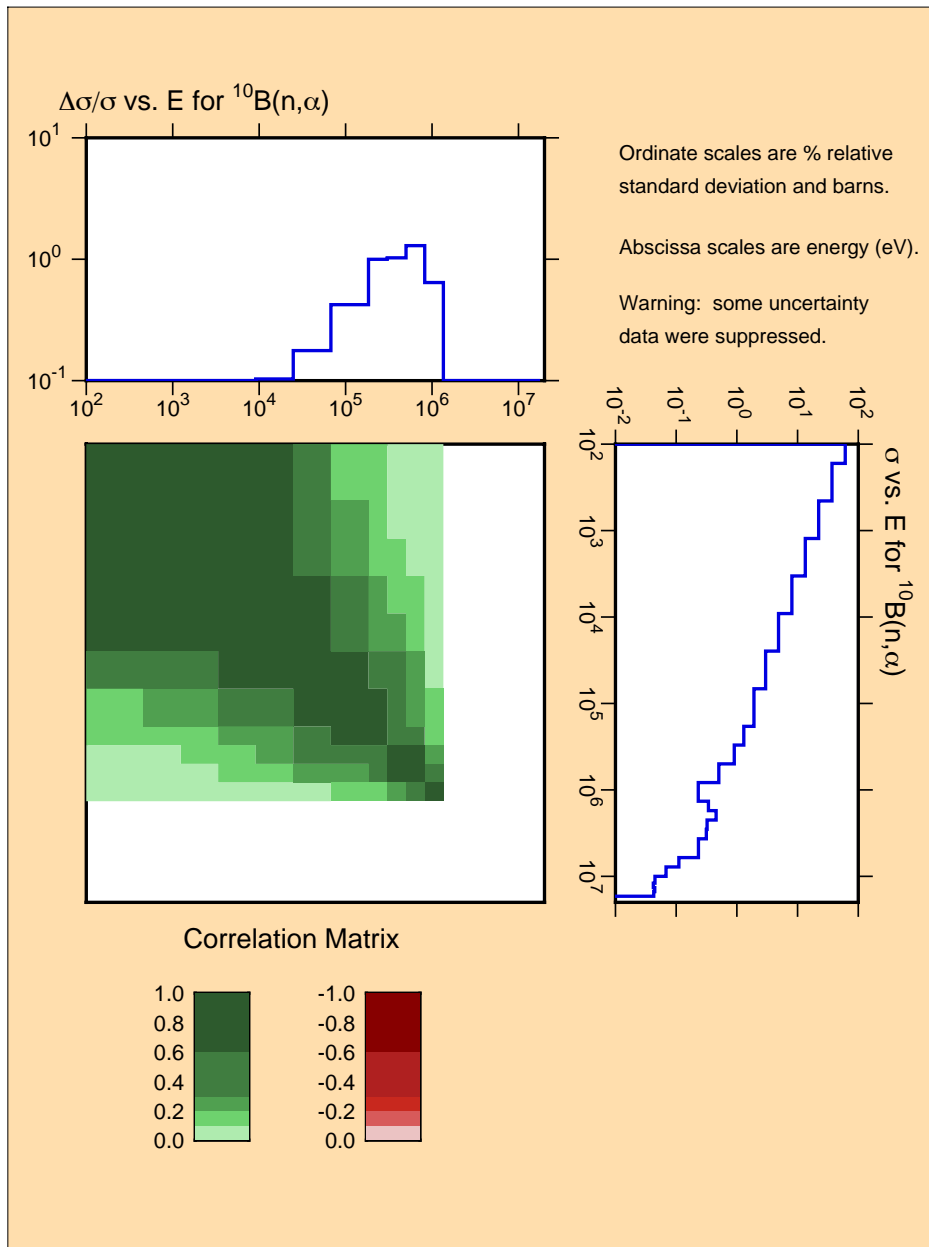
Figure 40: Covariance plot for ^{10}\text{B}(n,\alpha) from ENDF/B-VII.0. This reaction is used as a standard in the ENDF system.
