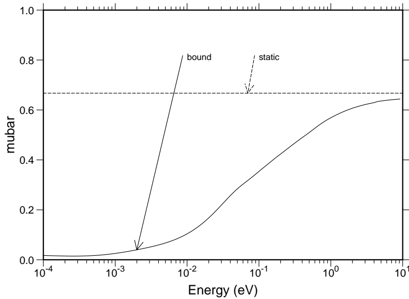
Figure 86: The average scattering cosine for H in H 2 O compared to the static value for scattering from atoms at rest. The effect of the binding of H in H 2 O is to make the scattering more isotropic at thermal energies.
