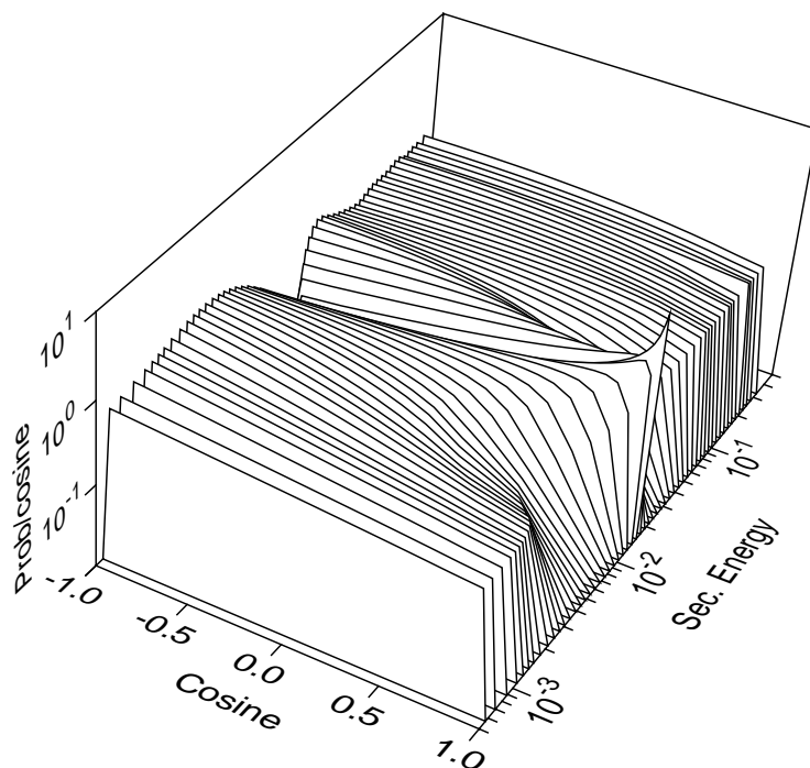
Figure 58: A perspective view of an angle-energy distribution for H in H 2 O.
