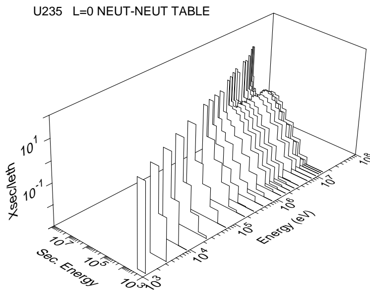
Figure 52: This plot shows the P_0 scattering matrix for ENDF/B-VI ^{235}\text{U} by incident and secondary energy.
