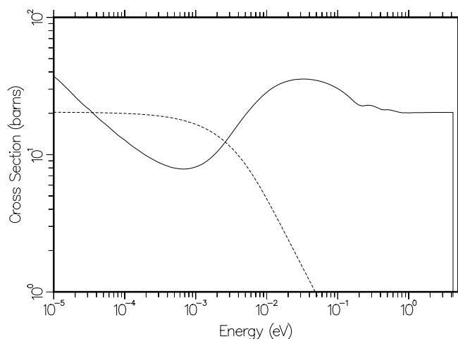
Figure 93: Inelastic (solid) and incoherent elastic (dashed) cross sections for solid methane. The small bumps starting at about 0.2 eV are due to the discrete levels at 0.162 eV, 0.190 eV, 0.361 eV, and 0.374 eV.
