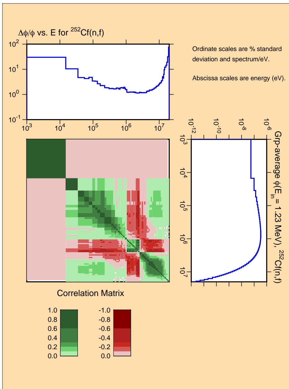
Figure 43: Example of energy distribution covariances. The appearance of negative correlations results from the requirement for preserving normalization.
