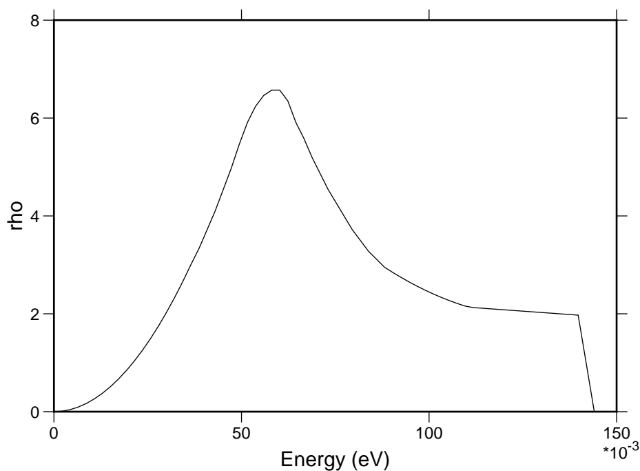
Figure 79: The frequency spectrum used for H in H 2 O for ENDF/B-VII.0.
