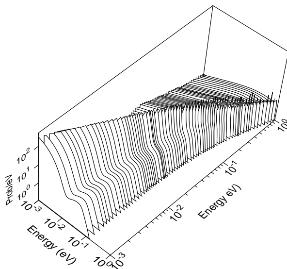
Figure 88: A perspective view of the isotropic part of the incoherent inelastic scattering from H in H 2 O. The variations in the size of the quasi-elastic peak are artifacts of the plotting program.
