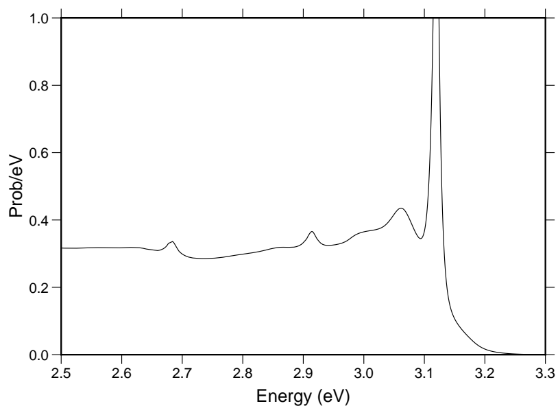
Figure 83: Detailed view of a neutron emission spectrum for inelastic scattering for H in \text{H}_2\text{O} .
