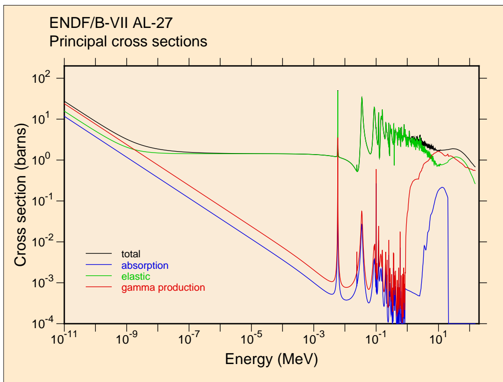
Figure 56: A log plot of the ACE principal cross sections for ^{27}\text{Al} from ENDF/B-VII.0. Note the extension beyond 20 MeV to 150 MeV.
