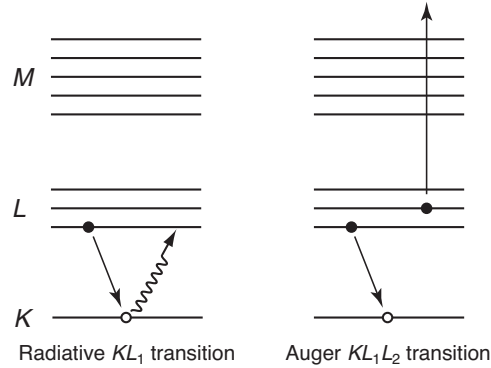
Figure 35: Definition of the KL and KLL notations for atomic relaxation.
