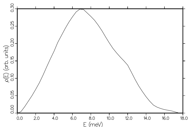
Figure 96: Effective frequency spectrum for methane including both translational and rotational modes, but not including diffusive modes.
