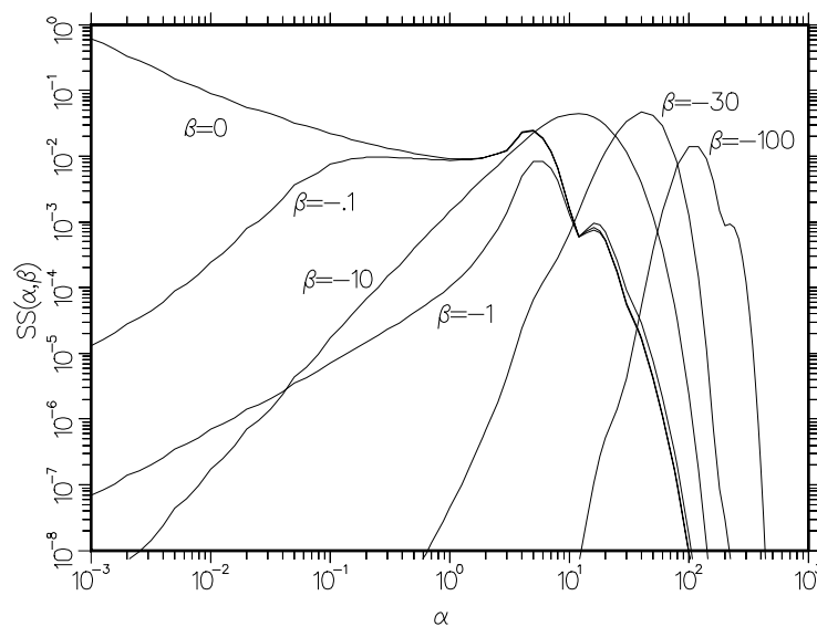
Figure 103: Script-S for para-hydrogen at 20K is shown as a function of \alpha for several \beta values corresponding to downscatter.
