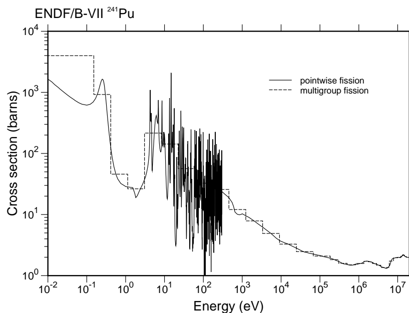
Figure 63: Comparison of the multigroup fission cross section of ENDF/B-VII.0 ^{241}\text{Pu} (dashed curve) with the corresponding pointwise cross section from the PENDF tape (solid curve).
