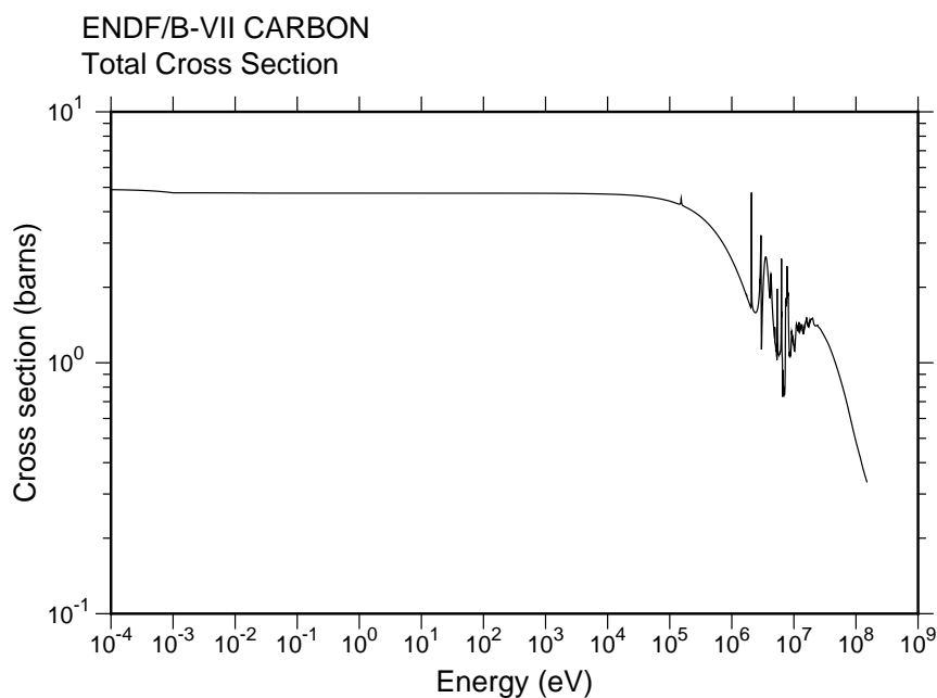
Figure 60: Simple 2-D plot of the total cross section of ENDF/B-VII carbon using automatic log-log axes.
