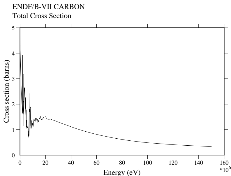
Figure 62: Simple 2-D plot of the total cross section of ENDF/B-VII.0 carbon using linear axes to emphasize the high-energy region and a more elaborate font.
