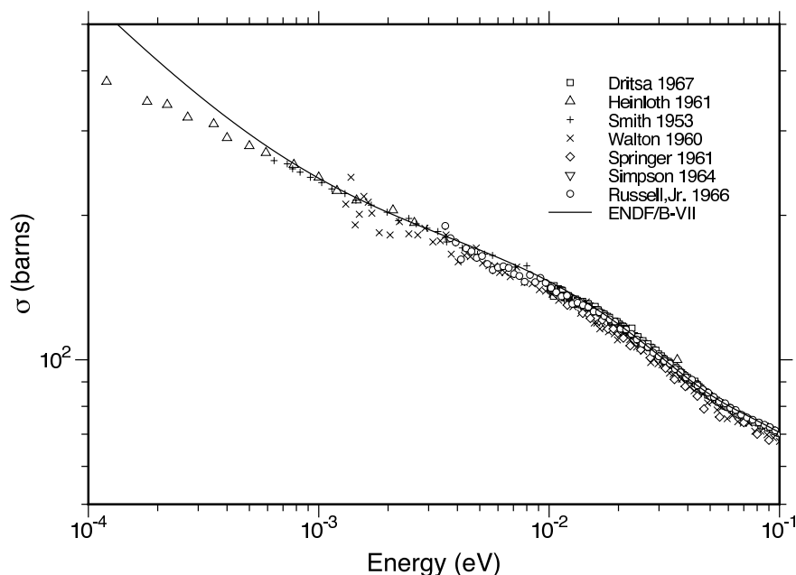
Figure 89: Comparison of the ENDF/B-VII.0 thermal cross section for water at lower incident energies with experimental results for the CSISRS compilation at the the National Nuclear Data Center of the Brookhaven National Laboratory. See the compilation for the references.
