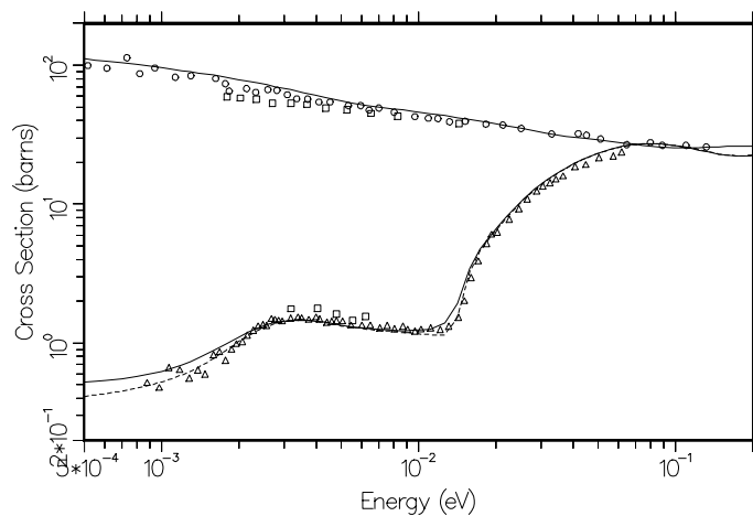
Figure 108: The cross sections for liquid ortho-hydrogen (upper curve) and liquid para-hydrogen (lower curve) at 20K are compared with experimental data[131] due to Squires (gas) at 20K (squares), Whittemore at 20K (circles), and Seiffert at 14K (triangles). The solid curves are at 20K and the dashed curve is at 14K. The sharp drop in the para cross section below 0.05 eV is due to spin coherence, and the second drop below 0.003 eV is due to intermolecular interference.
