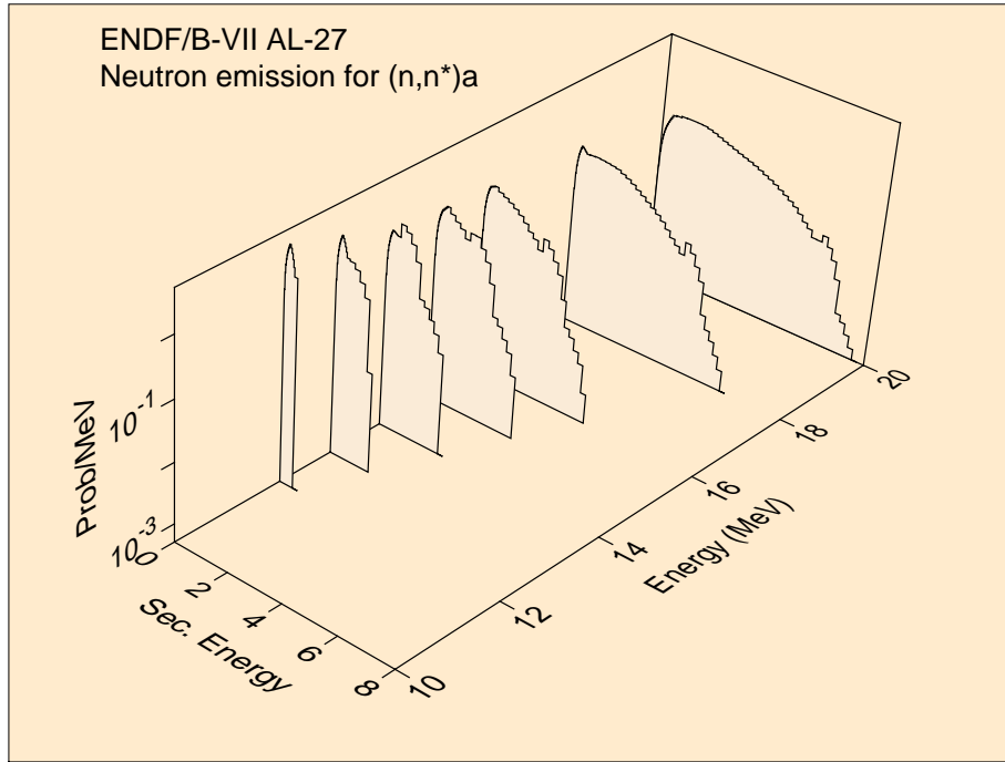
Figure 57: A 3-D view of the energy distribution for neutrons emitted from the (n,n'\alpha) reaction on ^{27}\text{Al} from ENDF/B-VII.
