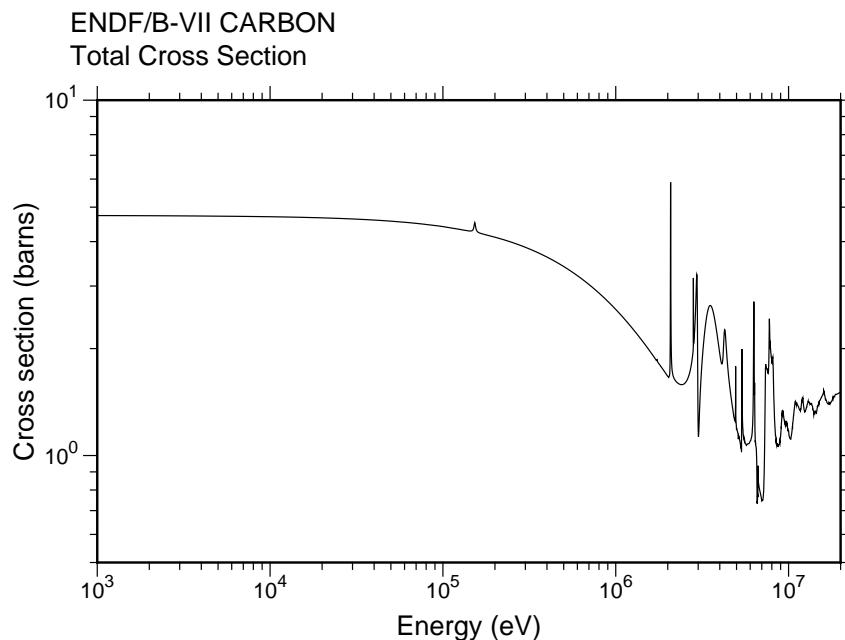
Figure 61: Simple 2-D plot of the total cross section of ENDF/B-VII carbon using log-log axes with user-selected ranges.
