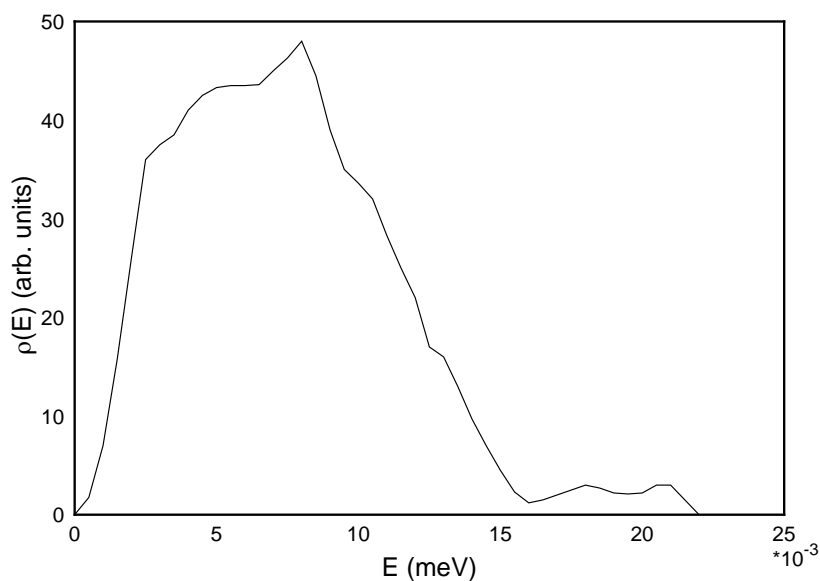
Figure 91: The Harker-Brugger frequency spectrum used for solid methane. Note the quadratic shape at low energies.
