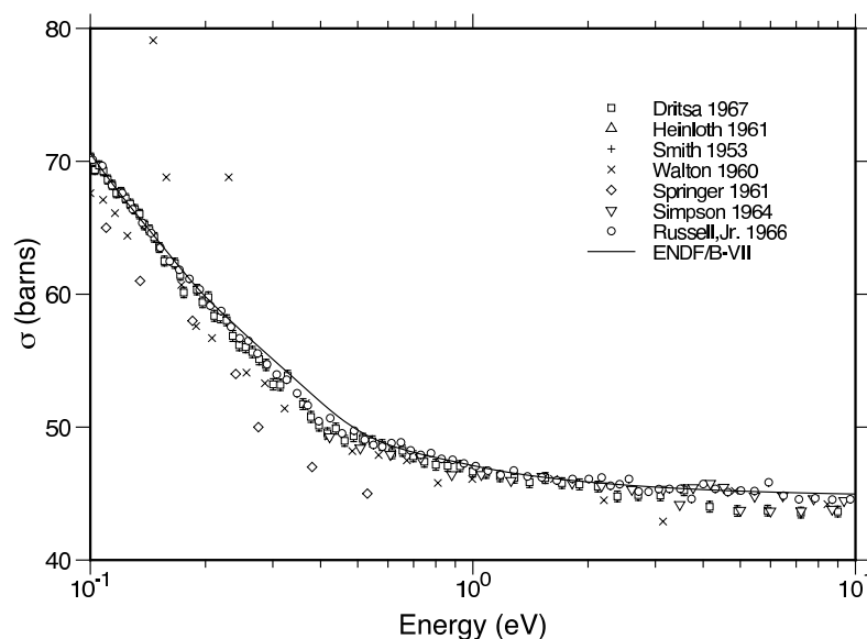
Figure 90: Comparison of the ENDF/B-VII.0 thermal cross section for water at higher incident energies with experimental results for the CSISRS compilation at the the National Nuclear Data Center of the Brookhaven National Laboratory. See the compilation for the references.
