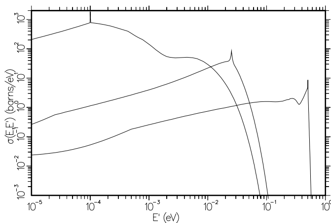
Figure 99: Neutron spectra \sigma(E \rightarrow E') are shown for E = 0.0001 eV, 0.0253 eV, and 0.503 eV. Note the sharp quasi-elastic peak that results from the diffusive term in the theory used here.
