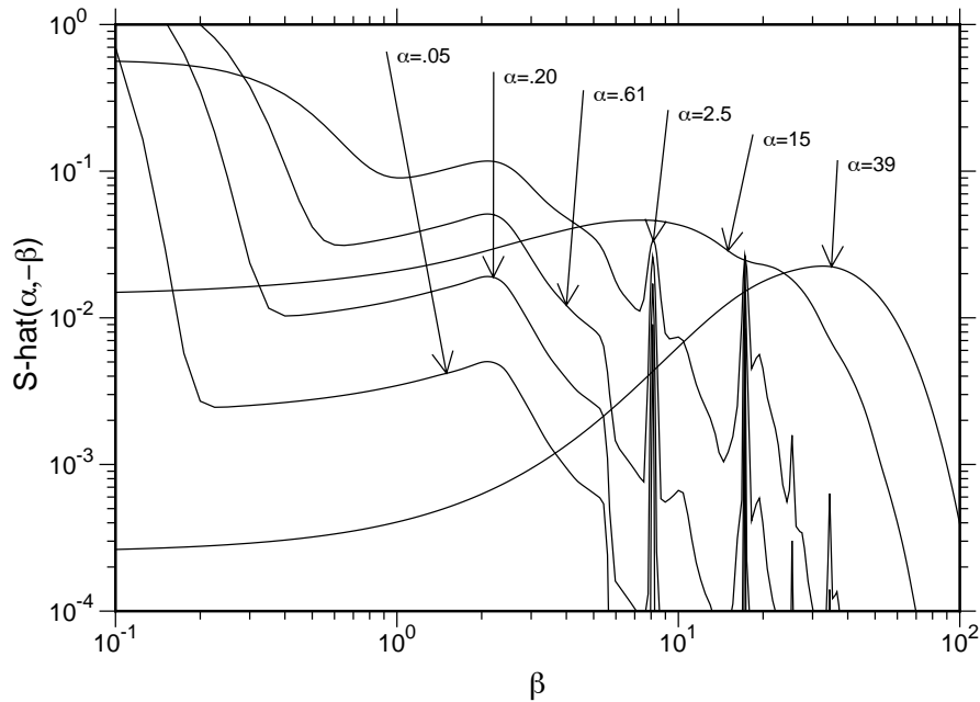
Figure 80: \mathcal{S}(\alpha, -\beta) for H in H 2 O at room temperature plotted versus \beta for various values of \alpha .
