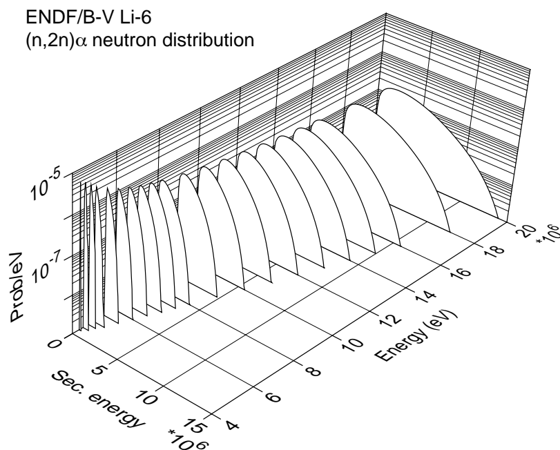
Figure 68: Perspective plot of {}^6\text{Li} (n,2n) \alpha neutron secondary-energy distributions.
