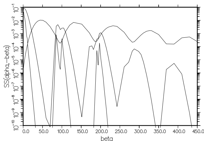
Figure 92: \mathcal{S}(\alpha, -\beta) for solid methane shown as a function of \beta for the \alpha values 0.986 (lowest), 16.94, and 151.45 (highest). The four discrete levels show up as sharp triangles in the lowest curve.
