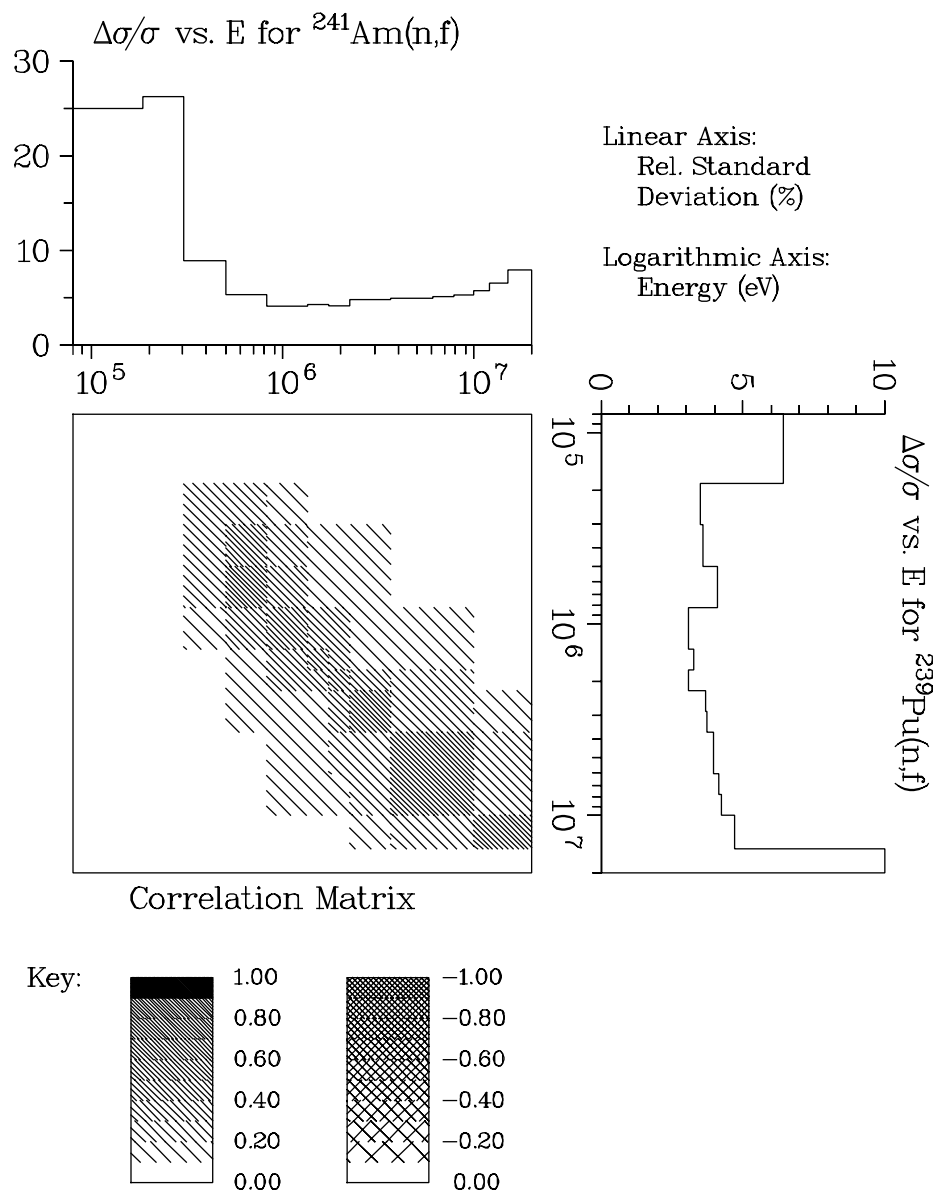
Figure 46: Covariance data for ^{239}\text{Pu}(n,f) with ^{241}\text{Am}(n,f) . This older figure illustrates the black & white option for covariance plots using hatching to represent levels of correlation.
