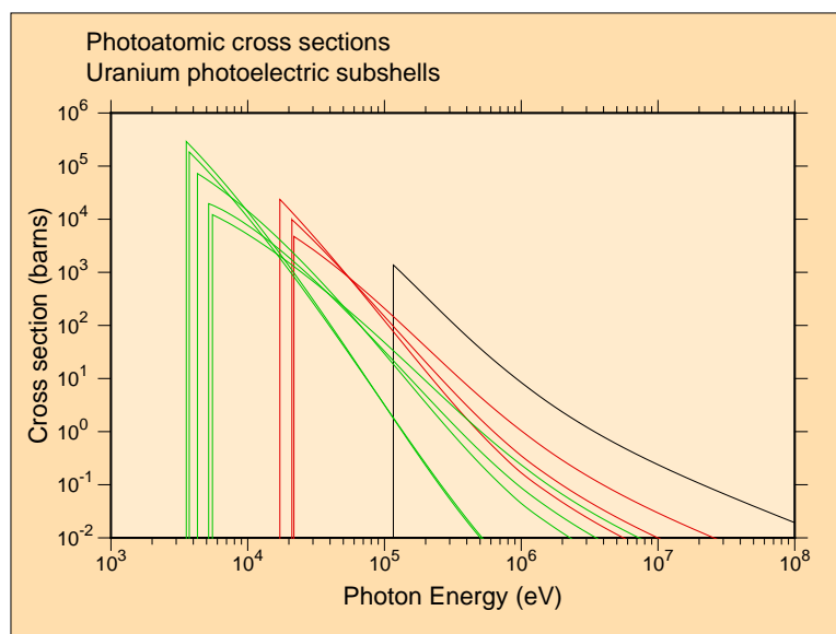
Figure 39: The first nine photoelectric subshell cross sections for uranium from ENDF/B-VII.0. Black is the S subshell ( 1s^{1/2} ), red is the L1, L2, and L3 subshells ( 2s^{1/2} , 2p^{1/2} , 2p^{3/2} ), and green is the M1 through M5 subshells ( 3s^{1/2} , 3p^{1/2} , 3p^{3/2} , 3d^{3/2} , 3d^{5/2} ).
