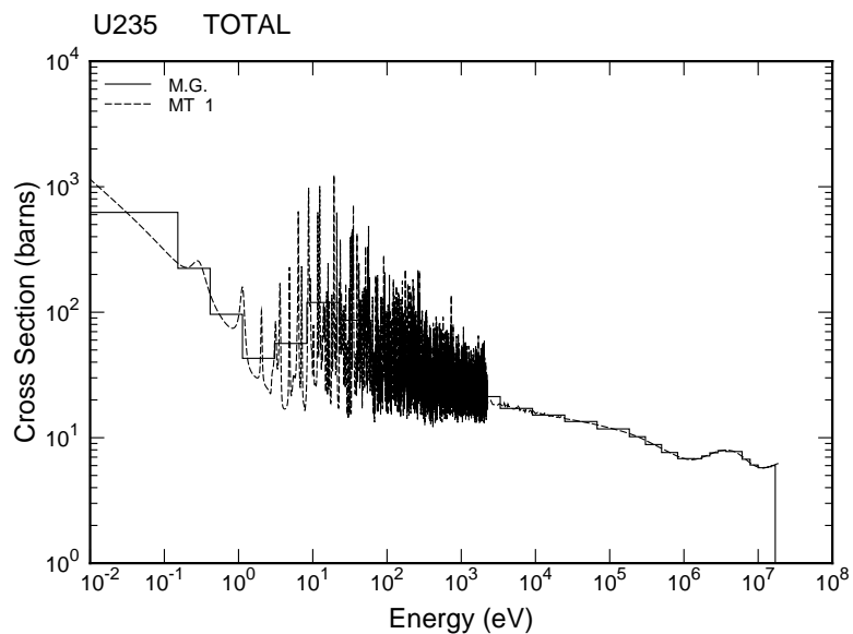
Figure 51: This is the total cross section for ENDF/B-VI ^{235}\text{U} from the same run as the previous plot. The energy range from 1 \times 10^{-5} eV to 1 \times 10^{-2} eV was removed to expand the rest of the energy scale.
