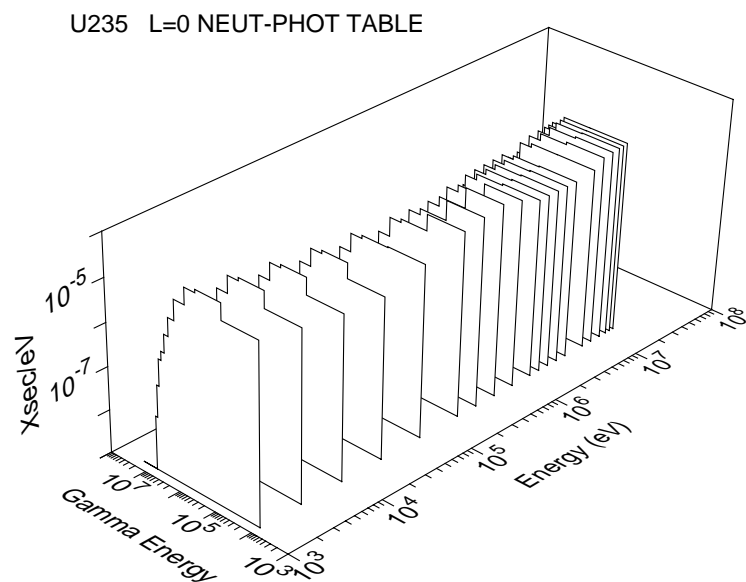
Figure 53: The 30 \times 12 P_0 photon production matrix for ^{235}\text{U} is plotted versus neutron energy and photon energy.
