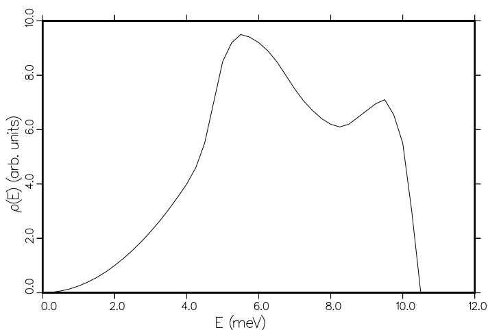
Figure 100: The Keinert-Sax frequency distribution for the effective translational modes of liquid hydrogen.
