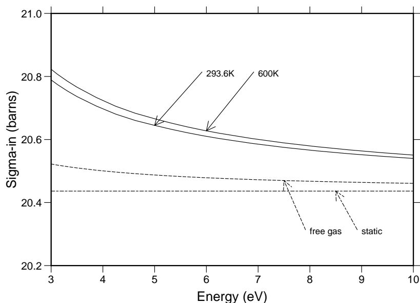
Figure 85: The incoherent inelastic cross section for H in \text{H}_2\text{O} for higher incident energies showing the static limit (scattering from atoms at rest) and the free-gas cross section.
