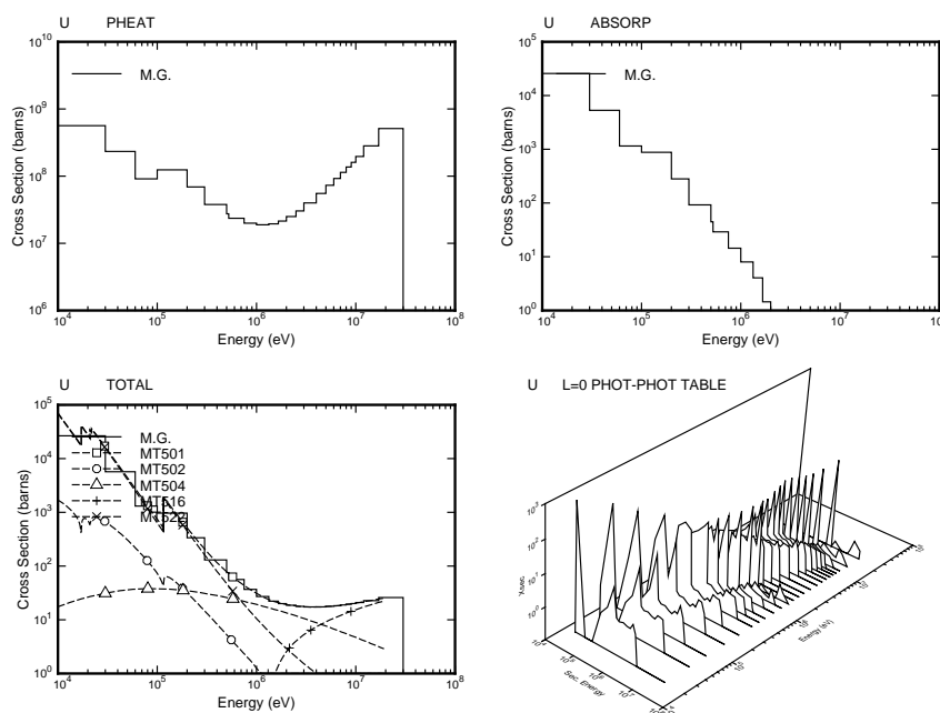
Figure 37: Plots of the photon interaction cross sections and the photon scattering distribution for uranium showing both 24-group and continuous cross sections. Note the prominent photoelectric absorption edge near 100 keV.
