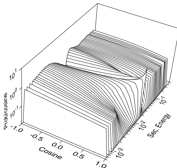
Figure 87: A perspective view of an angle-energy distribution for H in H 2 O.
