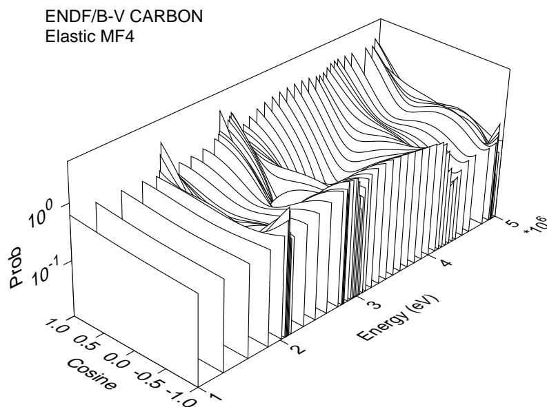
Figure 67: Perspective view of carbon elastic scattering angular distribution.
