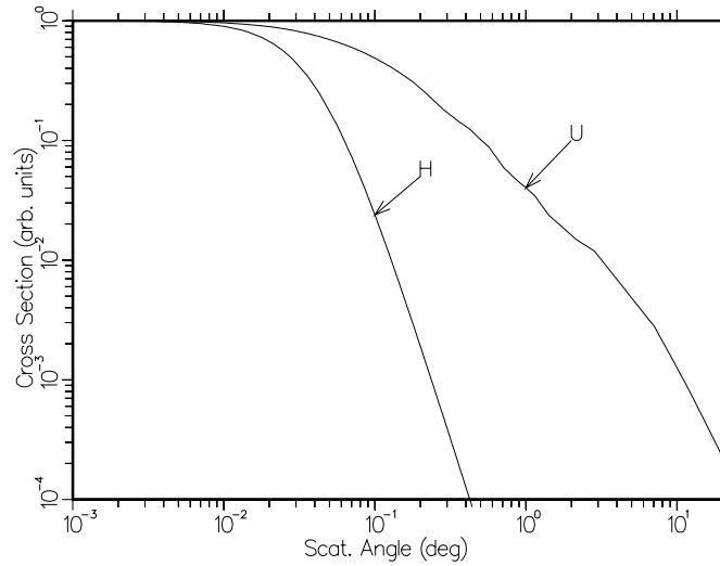
Figure 36: Angular distribution for coherent scattering from hydrogen and uranium at high photon energy.
