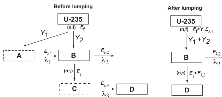
Figure 59: Lumping short-lived fission products in ^{235}\text{U} .
