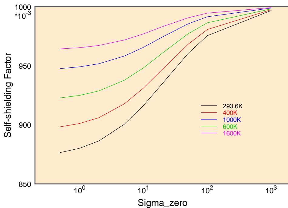
Figure 74: Self-shielding factors for the total cross section of ^{238}\text{U} at 20 keV showing the variation with temperature and background cross section (dilution).
