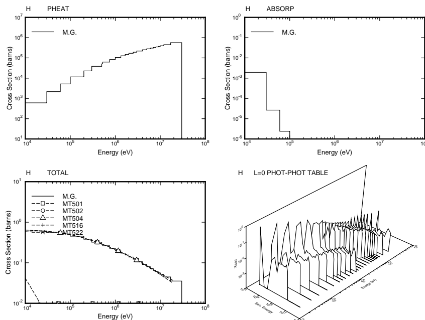
Figure 38: Plots of the photon interaction cross sections and the photon scattering distribution for hydrogen showing both 24-group and continuous cross sections. The cross sections are simpler for this case.
