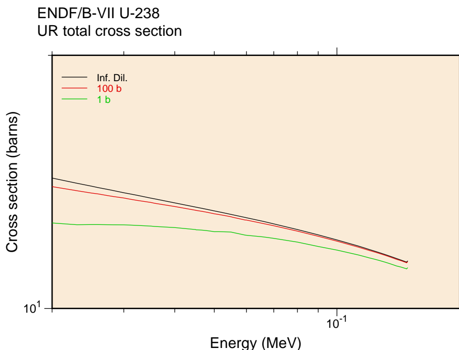
Figure 73: Bondarenko-style self-shielded cross sections for the total cross section of ^{238}\text{U} in the unresolved resonance region at three different dilutions.
