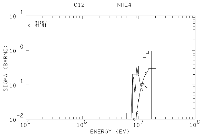
Figure 55: An example of a DTFR edit plot showing multiple pointwise curves that are the components of a compound edit. This graph is for ENDF/B-IV ^{12}\text{C} helium production. The histogram gives the sum of the (n,\alpha) cross section and three times the (n,n')3\alpha cross section.
