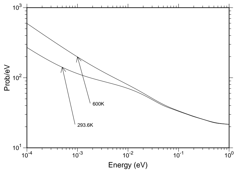
Figure 84: The incoherent inelastic cross section for H in \text{H}_2\text{O} at two temperatures.
