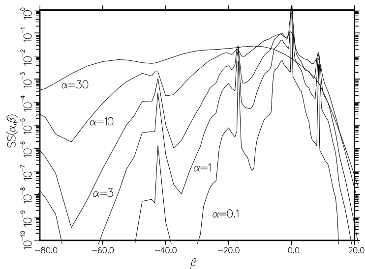
Figure 104: Script-S for ortho-hydrogen at 20K is shown as a function of \beta for several \alpha values.
