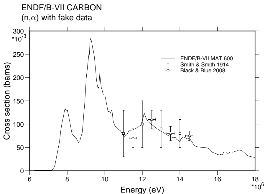
Figure 66: Carbon (n, \alpha ) cross section compared with two sets of simulated experimental data represented with two types of error bars.
