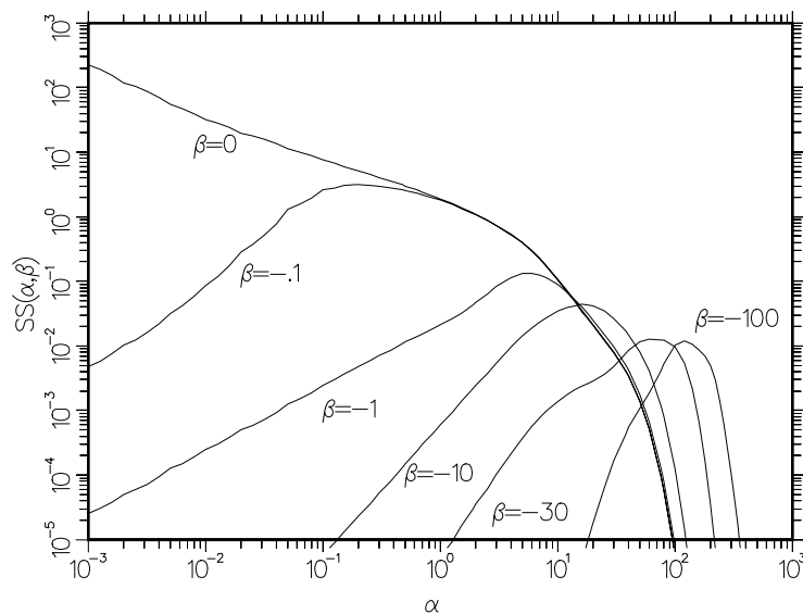
Figure 105: Script-S for ortho-hydrogen at 20K is shown as a function of \alpha for several \beta values corresponding to downscatter.
