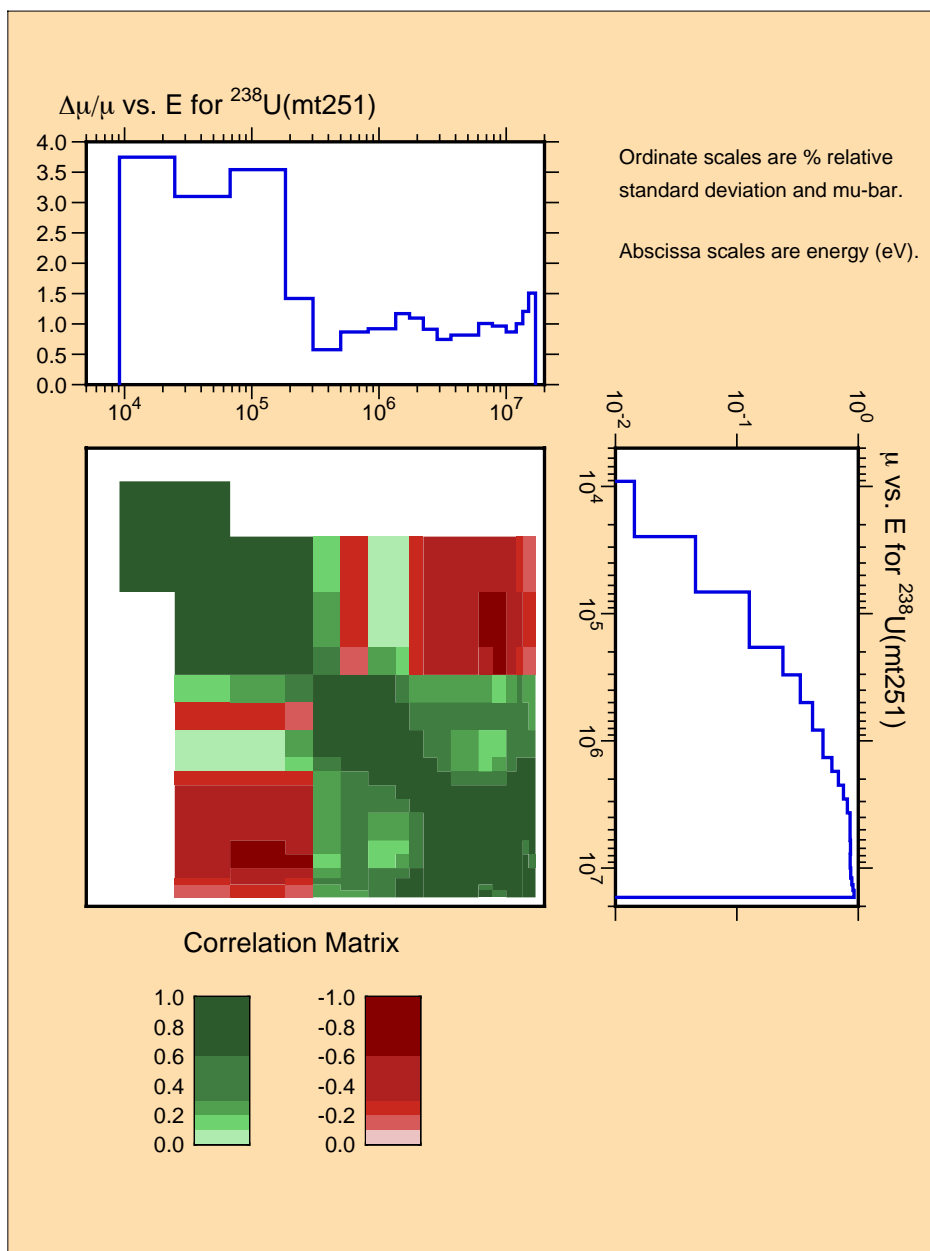
Figure 42: Example of angular distribution covariance data.
