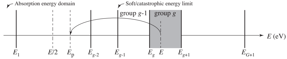
Figure 34: Definition of the arbitrary soft/catastrophic energy limit and of the absorption energy domain below E_1 .
