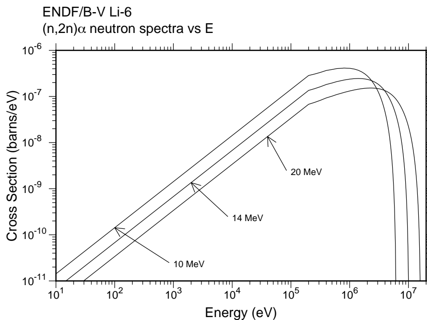
Figure 69: Two-D plot of selected secondary neutron spectra for the {}^6\text{Li} (n,2n) \alpha reaction.
