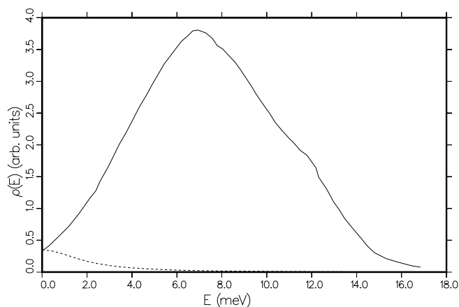
Figure 95: Frequency spectrum for liquid methane (solid) as given by Agrawal and Yip, including an analytic translational part (dashed) and a rotational part based on Gordon's analysis of the optical measurements of Ewing.
