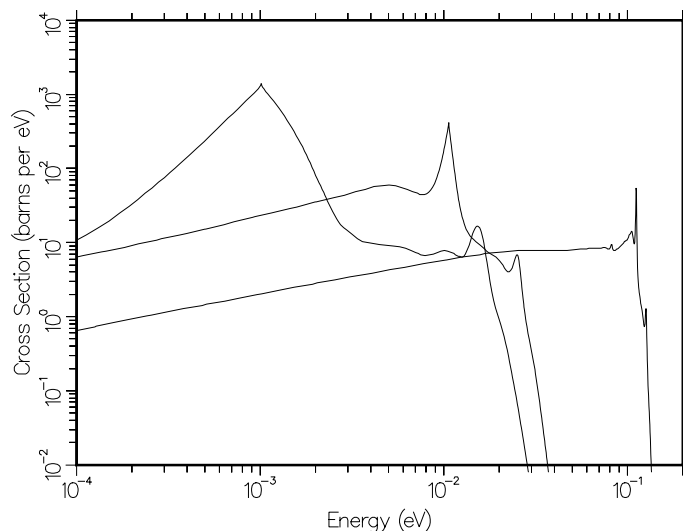
Figure 107: The spectra \sigma(E \rightarrow E') for liquid ortho-hydrogen are shown for E = 0.0001 eV, 0.0106 eV, and 0.112 eV.
