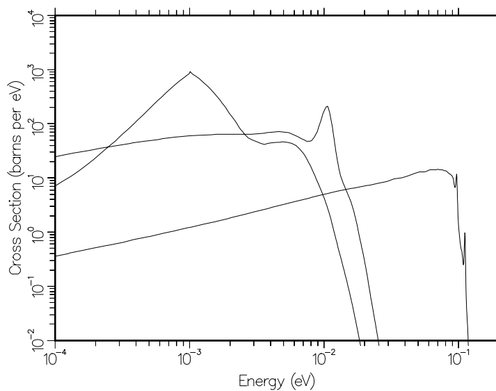
Figure 106: The spectra \sigma(E \rightarrow E') for liquid para-hydrogen are shown for E = 0.0001 eV, 0.0106 eV, and 0.112 eV.
